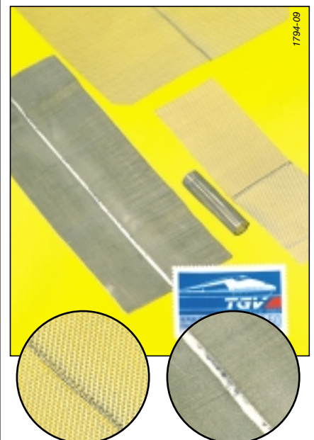
Welding metal fabric and mesh (expanded metal).
