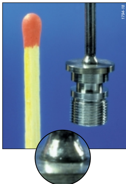
Tube welded to stainless steel union.
